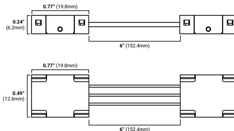
Uni-CCT-3P-TT-6W-12 (Tape-to-tape snap connector with 6" wire)
