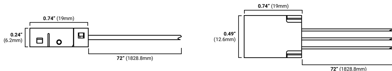
Uni-CCT-3P-TW-72W-12 (Tape to wire snap connector with 72" wire)
