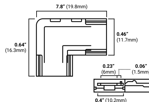
Uni-CCT-3P-LL-12 (Tape to tape L Shape 90° snap connector)
