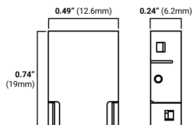
Uni-CCT-3P-TW-12 (Tape to wire snap connector)
