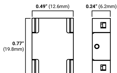
Uni-CCT-3P-TT-12 (Tape to tape snap connector)
