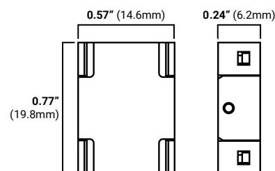
Uni-6P-TT-12 (Tape-to-tape snap connector)
