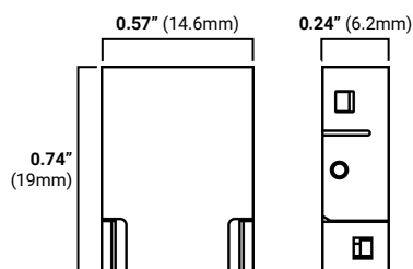
Uni-6P-TW-12 (Tape-to-wire snap connector)
