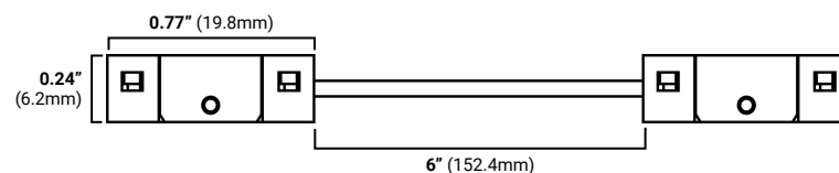
Uni-6P-TT-6W-12 (Tape-to-tape snap connector with 6" wire)
