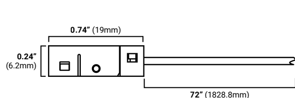
Uni-6P-TW-72W-12 (Tape-to-wire snap connector with 72" wire)
